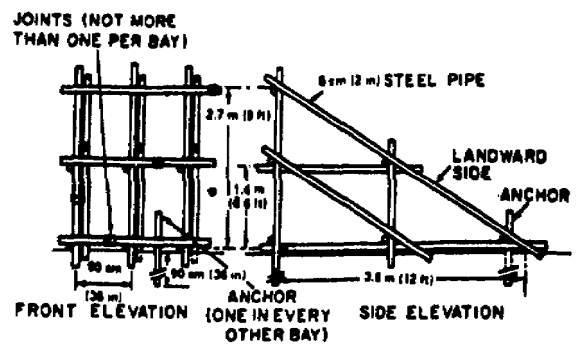
Figure 3-29. Steel scaffolding.
